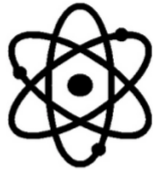
Atom
